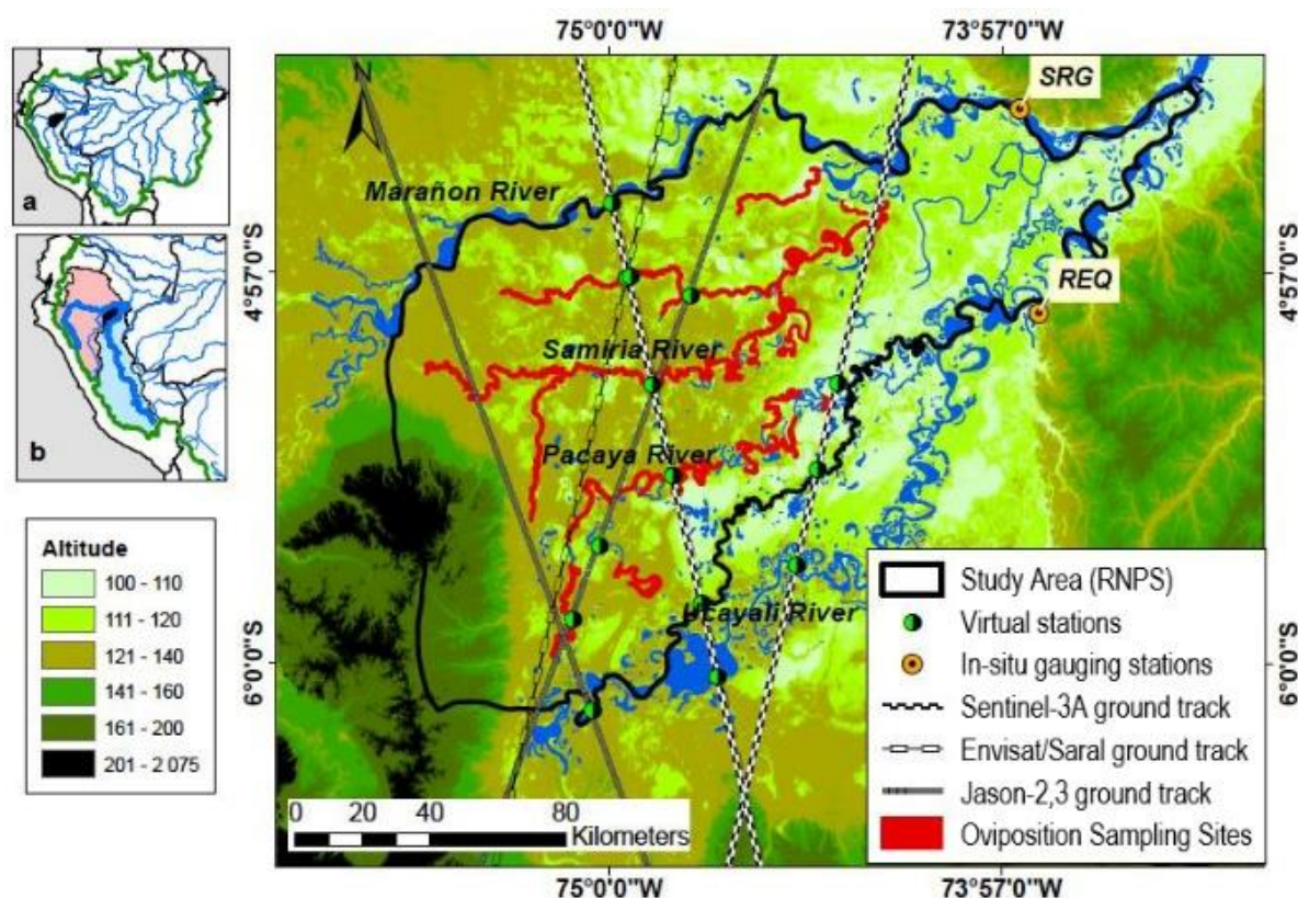
Figure 1. Study area with satellite trajectories location of virtual stations in situ water level gauge stations (SRG, REQ) in the Ucayali and Marañon rivers, and oviposition sampling areas. (Projection: GCS WGS 84 UTM 18S). (a) Amazon Basin in green border with the study area Pacaya Samiria National Reserve in black. (b) Peruvian Amazon Basin with the two major basins: Marañon Basin in pink with mainstem Marañon River and Ucayali Basin in blue with Ucayali River mainstem.
